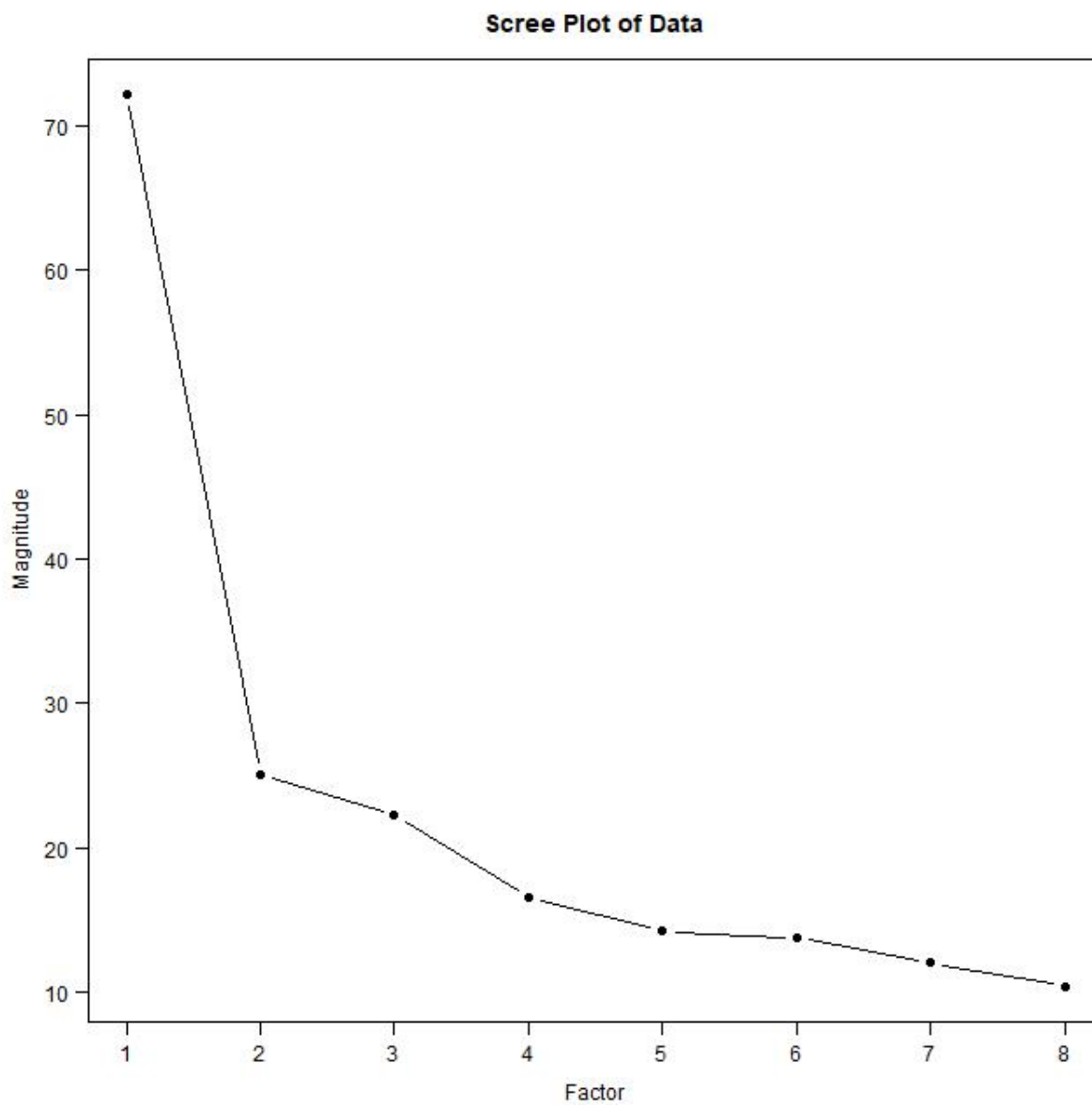
Figure S3: CCA scree plot after removing high-difficulty items with obscure truth values (A1, B2, B3, B4R), dichotomized following (M | O | A = 1, I | R | Q = 0), omitting four respondents with zero response variance.
