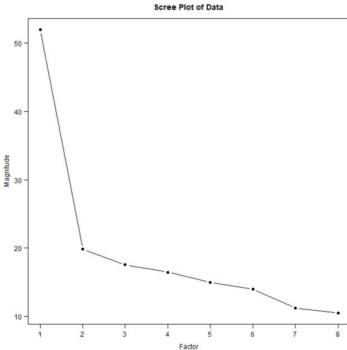
Figure S1: CCA scree plot based on all attributes, dichotomized following (M | O | A = 1, I | R | Q = 0), omitting two respondents with zero response variance.
