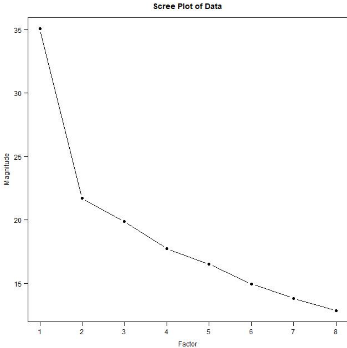
Figure S2: CCA scree plot based on all attributes, dichotomized following (M | O | A | R = 1, I | Q = 0), omitting three respondents with zero response variance.
